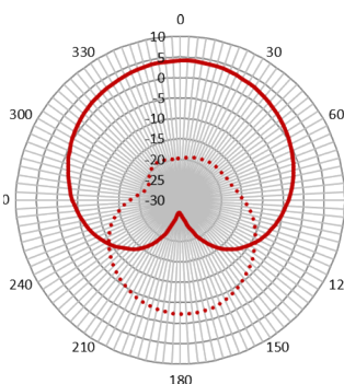
Vertical (FCC)
