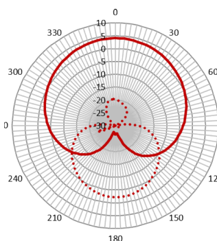
Horizontal (FCC)
