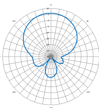
Horizontal (FCC)
